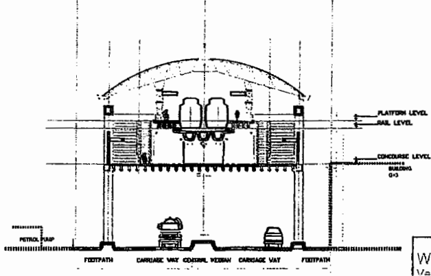
CROSS SECTION AT AA
