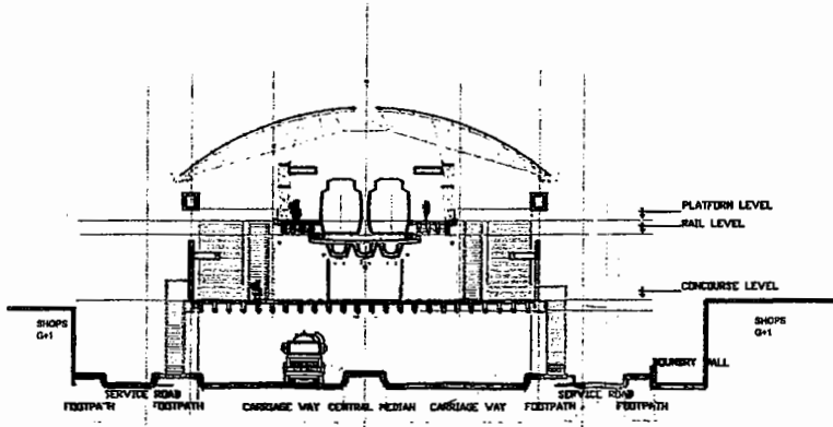
CROSS SECTION AT AA'
