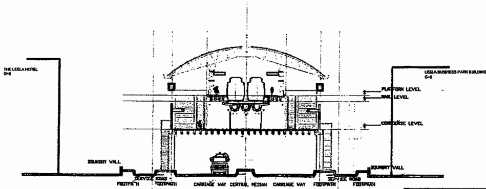
AIRPORT ROAD STATION Versova - Andheri - Ghatkoper Corridor East West MRTS Corridor Figure 7
