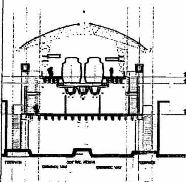
SECTION AT AA'
