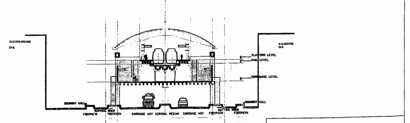
MAROL NAKA STATION Versova - Andheri - Ghatkopar East West MRTS Corridor Figure 8
