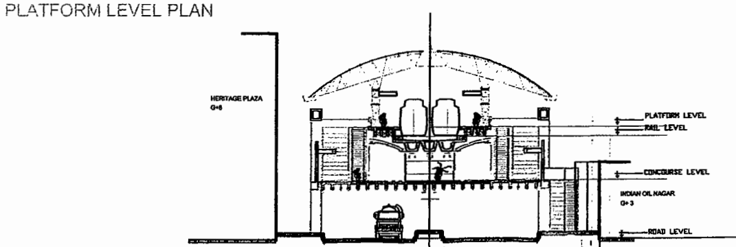
D N NAGAR STATION Versova - Andheri - Ghatkopar East West MRTS Corridor Figure 2
