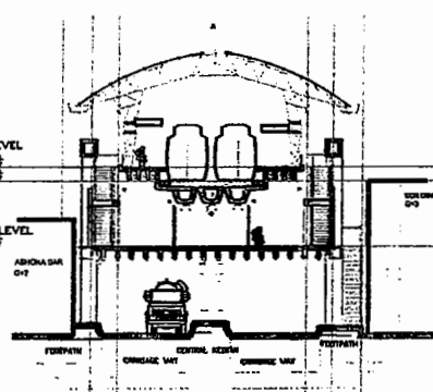
SECTION AT BB'
