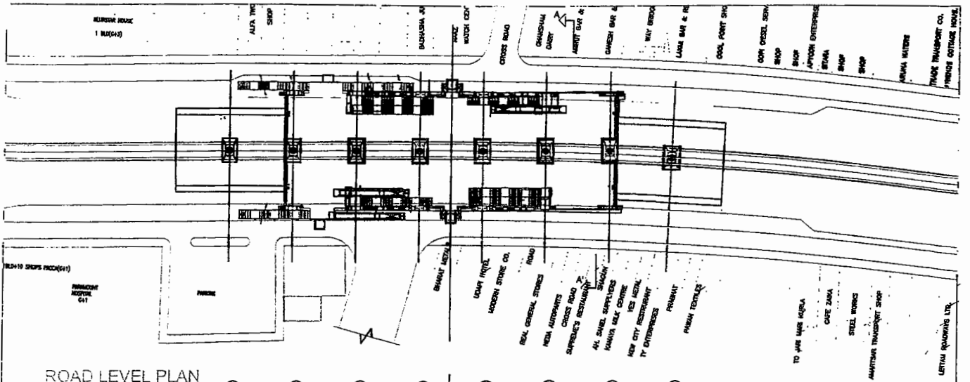
ROAD LEVEL PLAN
