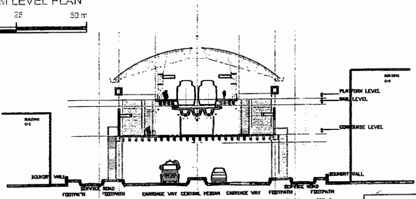
SUBHASH NAGAR STATION Versova - Andheri - Ghatkopar Corridor East West MRTS Corridor Figure 10
